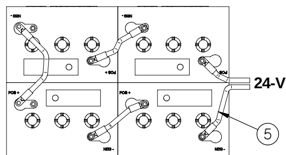
(4) 6-V BATTERY WIRING DIAGRAM
